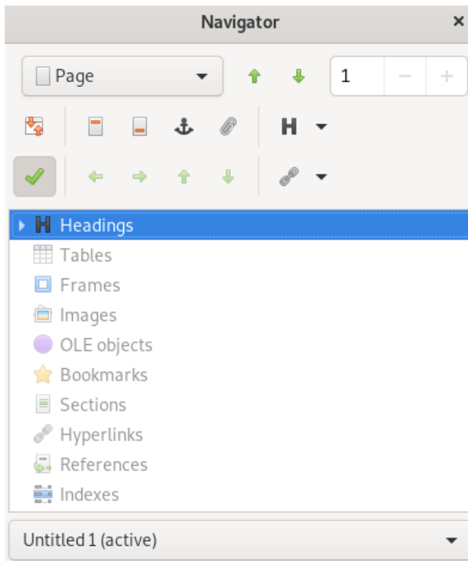
FIGURE 11.3: NAVIGATOR TOOL IN WRITER
